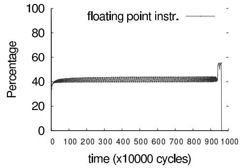
(b) ludcmp
