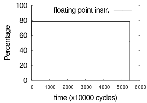
(f) syr2k
